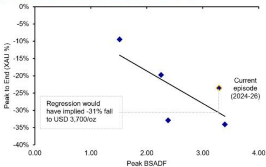
Figure 15: Gold depreciation from peak is also negatively related to peak BSADF statistic
