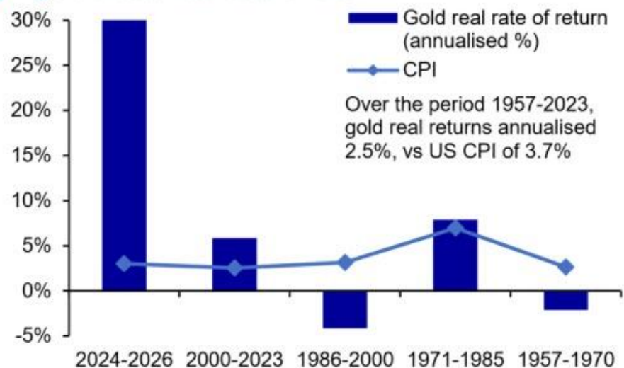
Figure 6: Gold real rates of return
