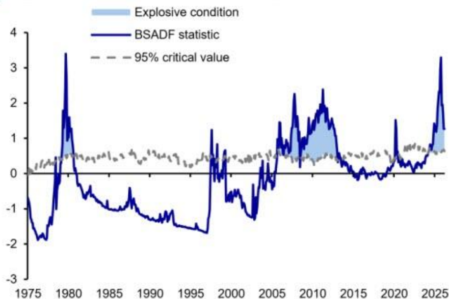
Figure 1: BSADF test statistic for gold since 1975
